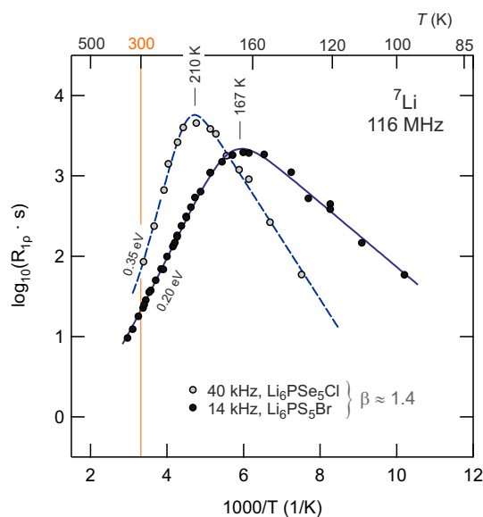
Figure 1: Arrhenius plot of the {}^7\text{Li} SLR NMR rates recorded with the spin-lock technique in the rotating frame of reference at frequencies of 14 kHz and 40 kHz, respectively; taken from Ref. [4]. The parameter \beta ( 1 < \beta \leq 2 ) indicates the deviation from ideal BPP-type behaviour [5] which would be reflected by \beta = 2 .
