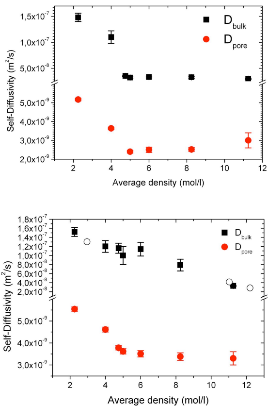
Fig.1 Self-diffusivity of ethane in bulk (squares) and in mesoporous silicon (circles) under sub-critical (top) and supercritical (bottom) conditions.
