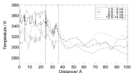
Fig. 2 Temperature profile as a function of the distance from the center of the zeolite during different periods of the second stage of the adsorption.
