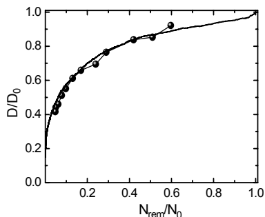
Fig. 1 Correlation plot of D/D_0 and N_{rem}/N_0 obtained for methane in zeolite NaCaA (35 \mu\text{m} crystal) (circles) with the corresponding theoretical curve (line). Visual comparison with the Monte Carlo simulation gives the value of the parameter \alpha R/5D_0 . The theoretical curve with \alpha R/5D_0=2 is found to provide the best fit to the experimental data and provides the permeability \alpha = (0.78 \pm 0.3) \times 10^{-3} \text{ m s}^{-1} .
