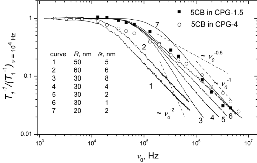
Figure 2. Normalised frequency dependencies of the spin-lattice relaxation rates, curves 1-7, evaluated from the simulated correlation functions. The curve parameter refers to different values of \delta r and R . The experimental data points refer to 5CB in CPG-1.5 and CPG-4 at 323 K.
