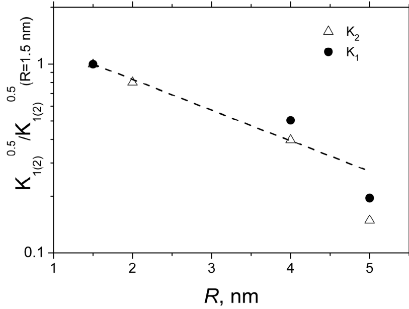
Figure 4. Normalised values of square root longitudinal ( K_1 ) and transverse ( K_2 ) relaxation rates of 5CB in pores as a function of the pore radius.
