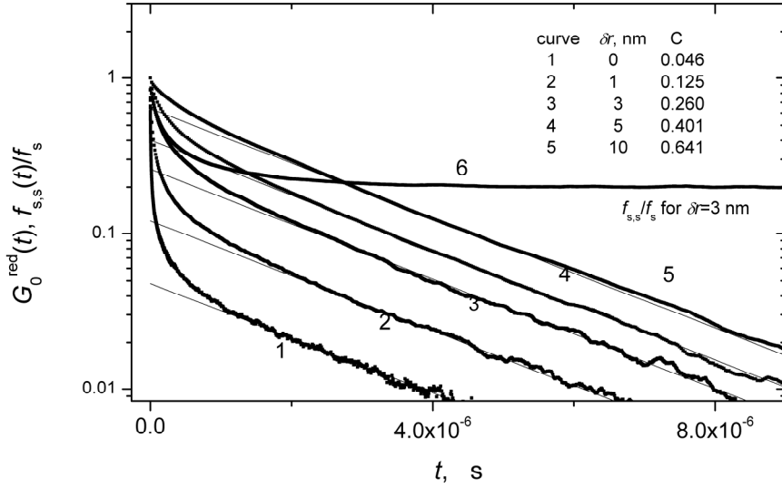
Figure 1. Monte Carlo simulations of the correlation function, Eq. (1), for k=0 , curves 1-5. The straight lines are fits of the function C \exp(-t/\tau_{RMTD}) to the long tails of the simulated functions. The values of C and \delta r are indicated in the inset. Curve 6 represents the (normalized) exchange-loss factor, f_{s,s}(t)/f_s , for \delta r = 3 nm.
