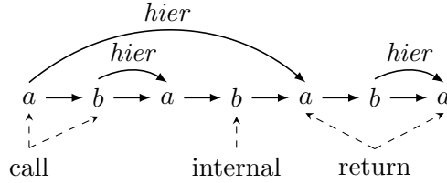
Figure 2.5: The graph representation of the finite nested word (abababa, \{(1, 5), (2, 3), (6, 7)\}) , which could also be written as \langle a\langle ba\rangle ba\rangle\langle ba\rangle . The linear edge labels lin were omitted.
